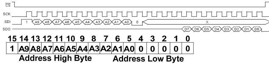
Figure 8. Long Address Read SPI Protocol
