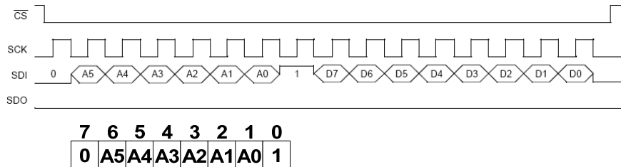
Figure 7. Short Address Write SPI Protocol
