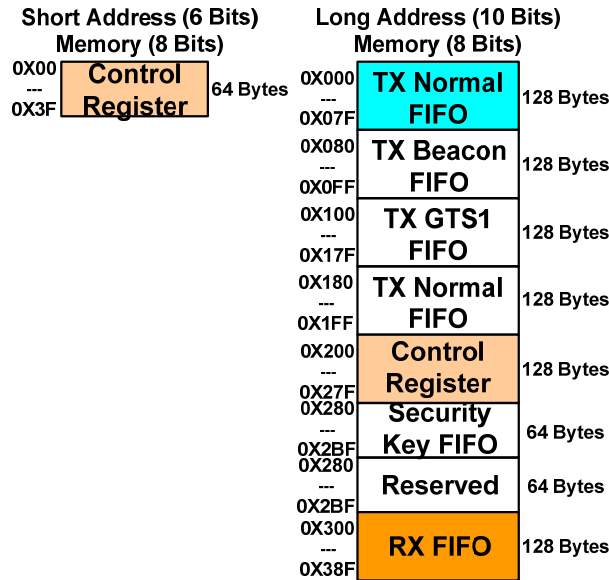
Figure 2. An Overview of the MRF24J40MA RAM Memory Map
