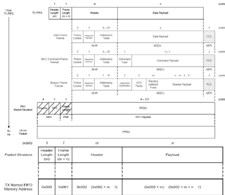
Figure 3. TX Normal FIFO Package Format
