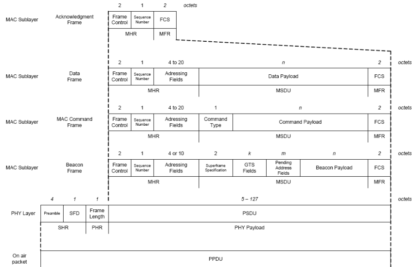
Figure 1. IEEE 802.15.4 Data Frame
