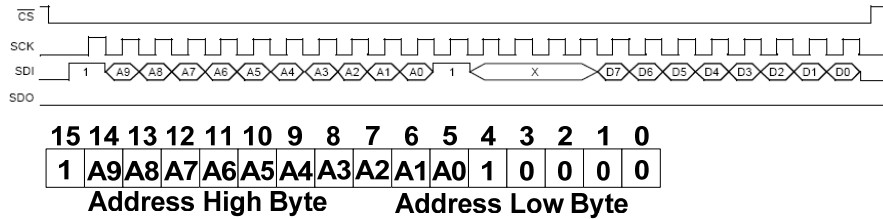
Figure 9. Short Address Read SPI Protocol
