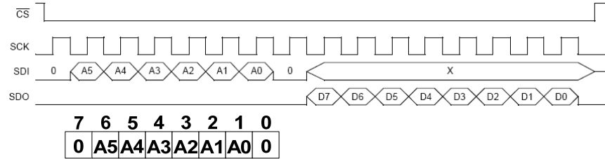
Figure 6. Short Address Read SPI Protocol
