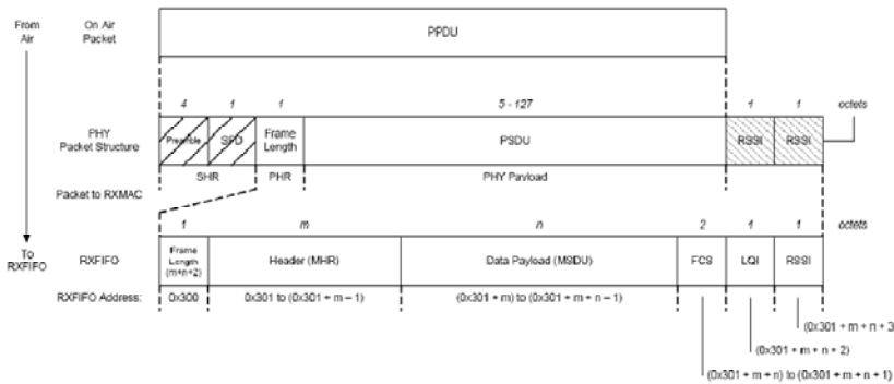
Figure 4. RX FIFO Package Format
