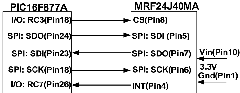
Figure 5. MRF24J40MA Module and Hardware Interface
